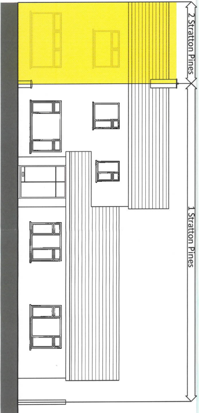
03 Proposed Front Elevation 210
